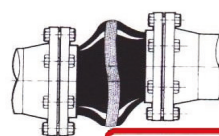
Fig. 3: 橫向偏移 Lateral Movement
